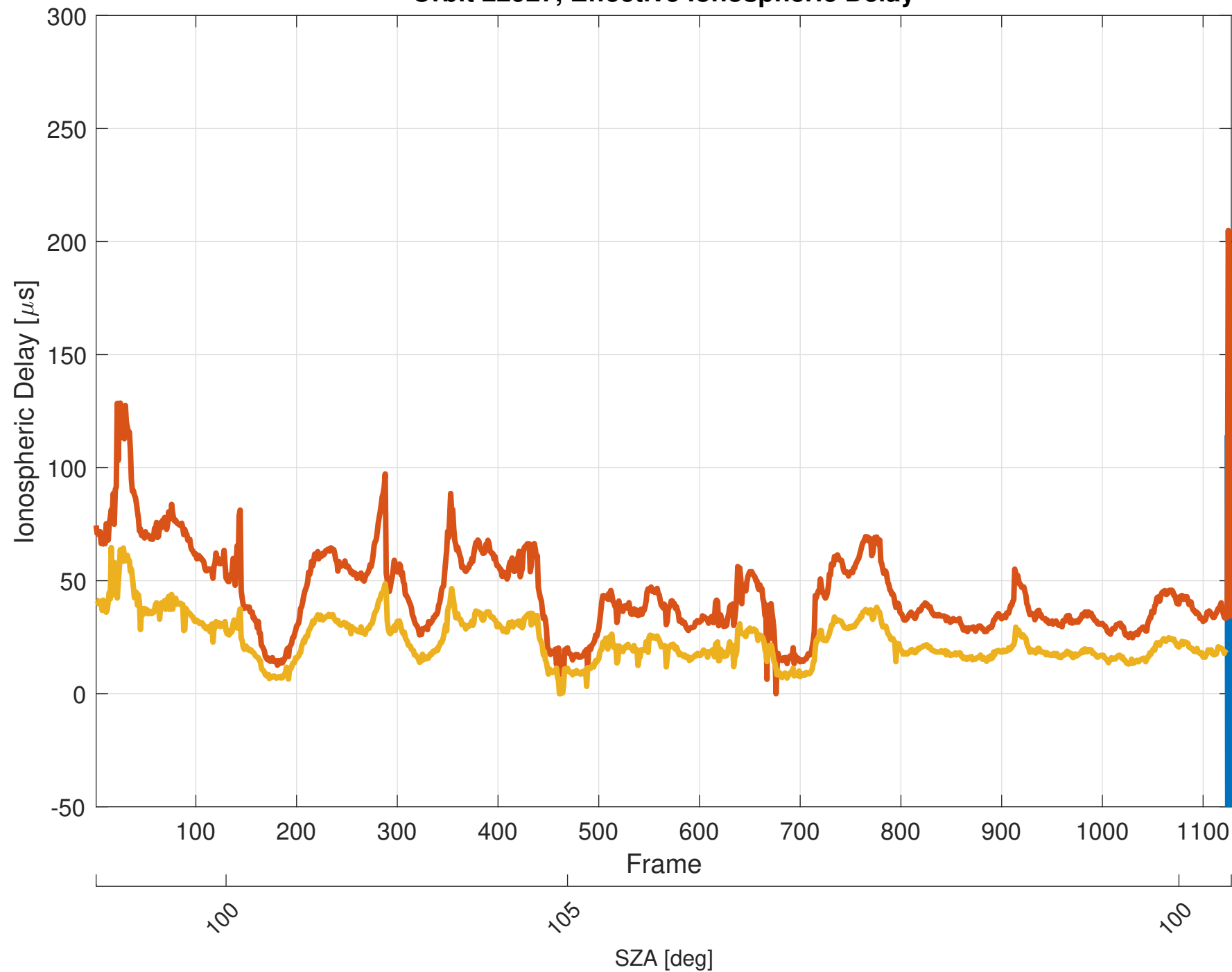
Orbit 22927, Effective Ionospheric Delay
