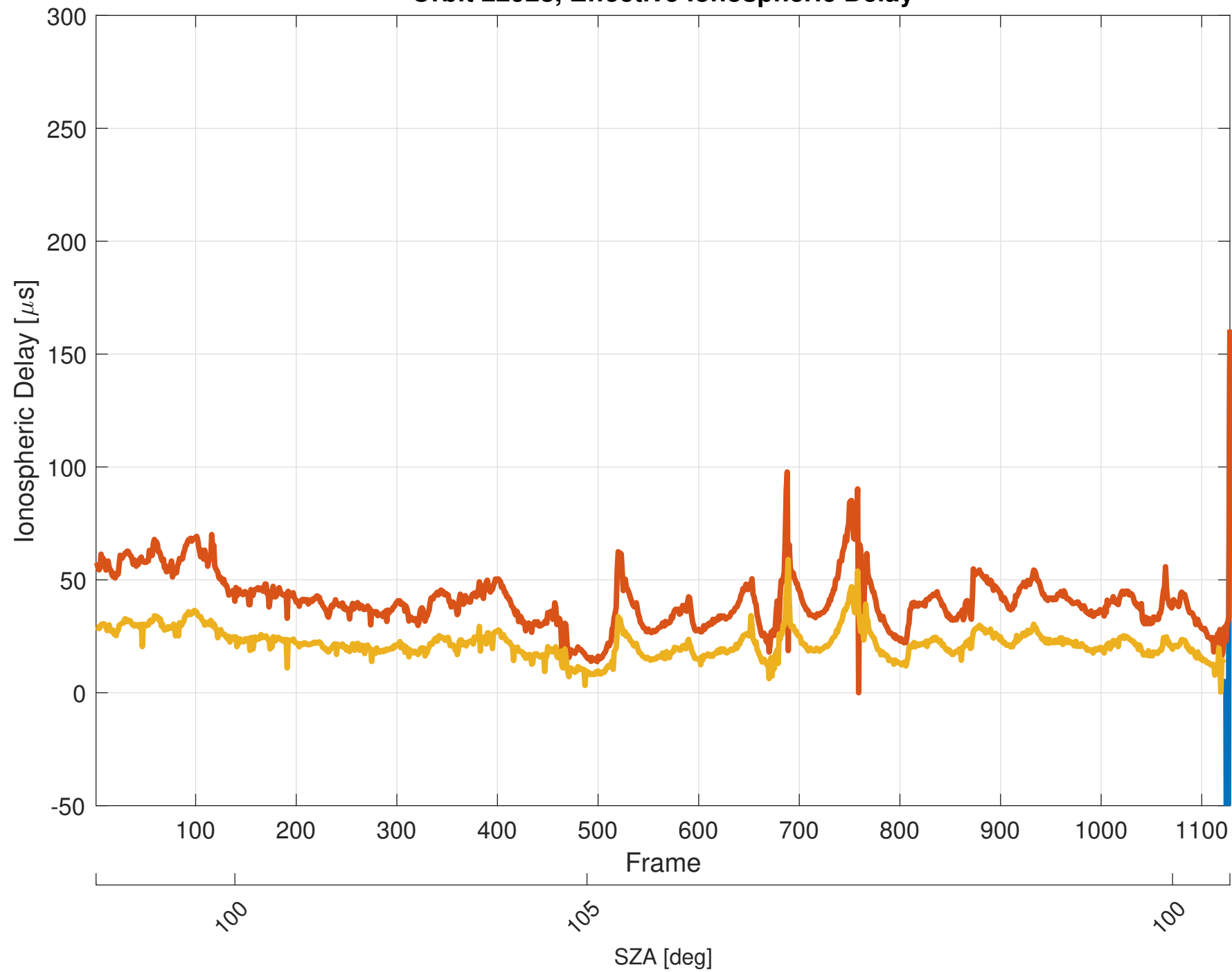
Orbit 22928, Effective Ionospheric Delay
