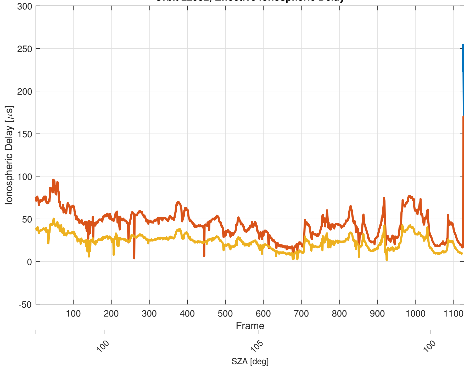
Orbit 22932, Effective Ionospheric Delay
