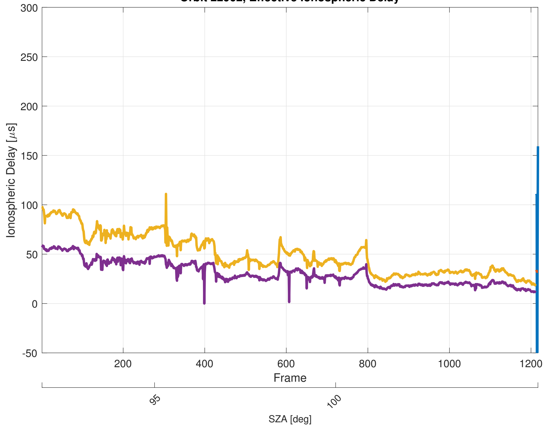
Orbit 22962, Effective Ionospheric Delay
