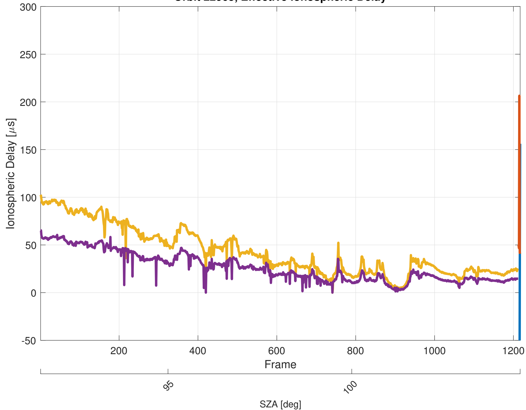
Orbit 22965, Effective Ionospheric Delay
