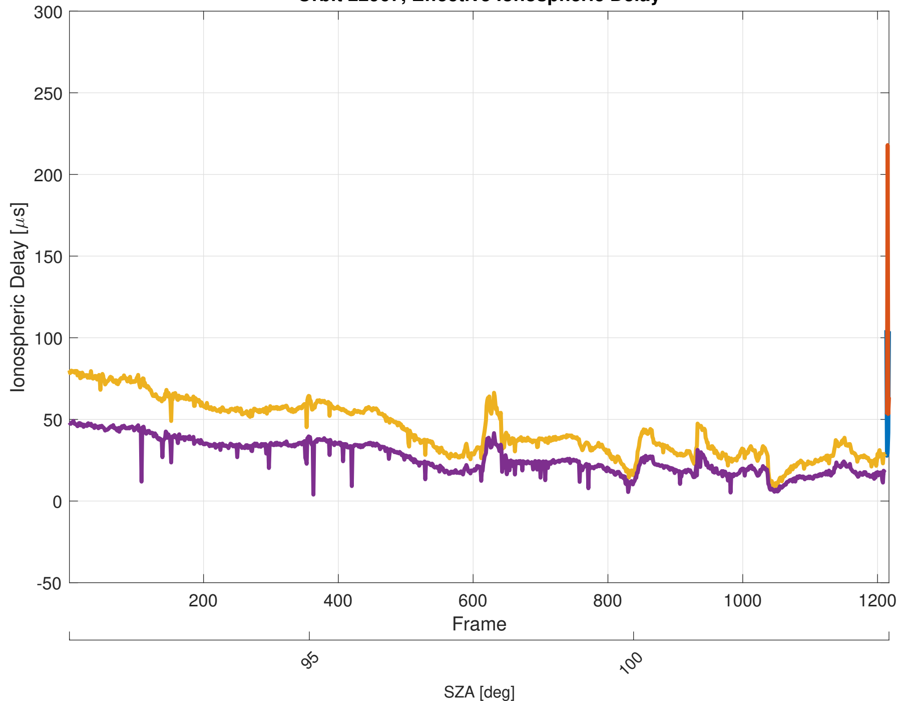
Orbit 22967, Effective Ionospheric Delay
