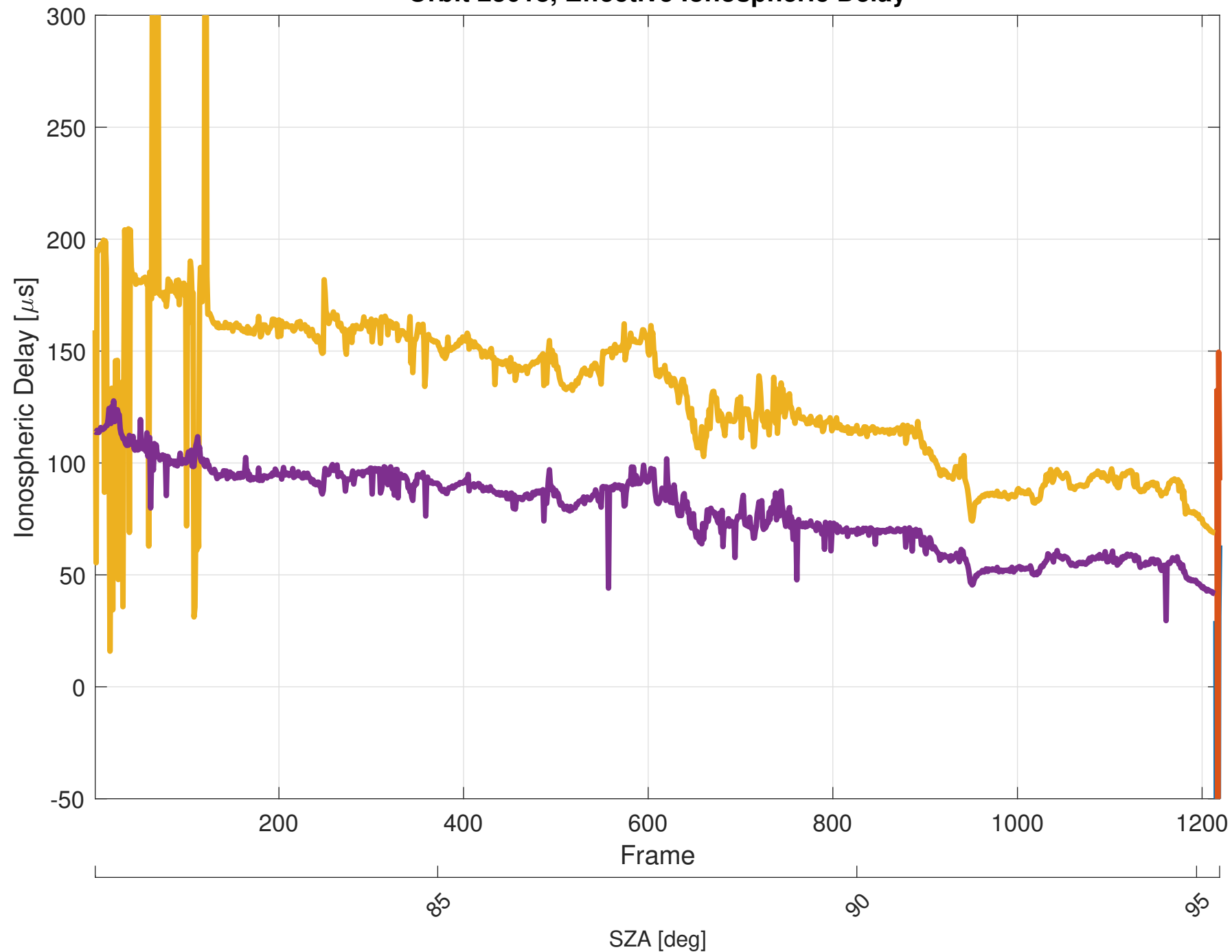
Orbit 23018, Effective Ionospheric Delay
