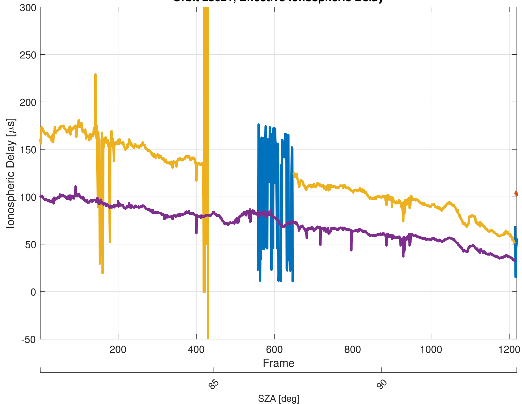
Orbit 23021, Effective Ionospheric Delay
