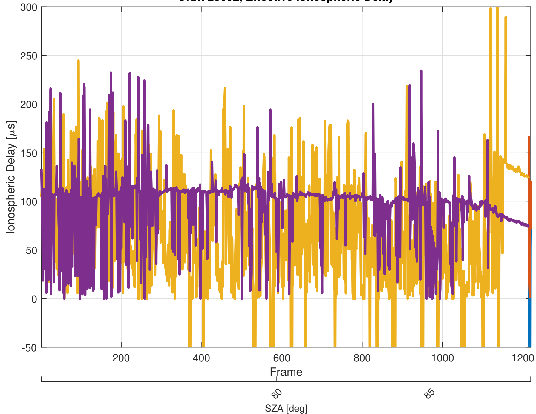
Orbit 23052, Effective Ionospheric Delay
