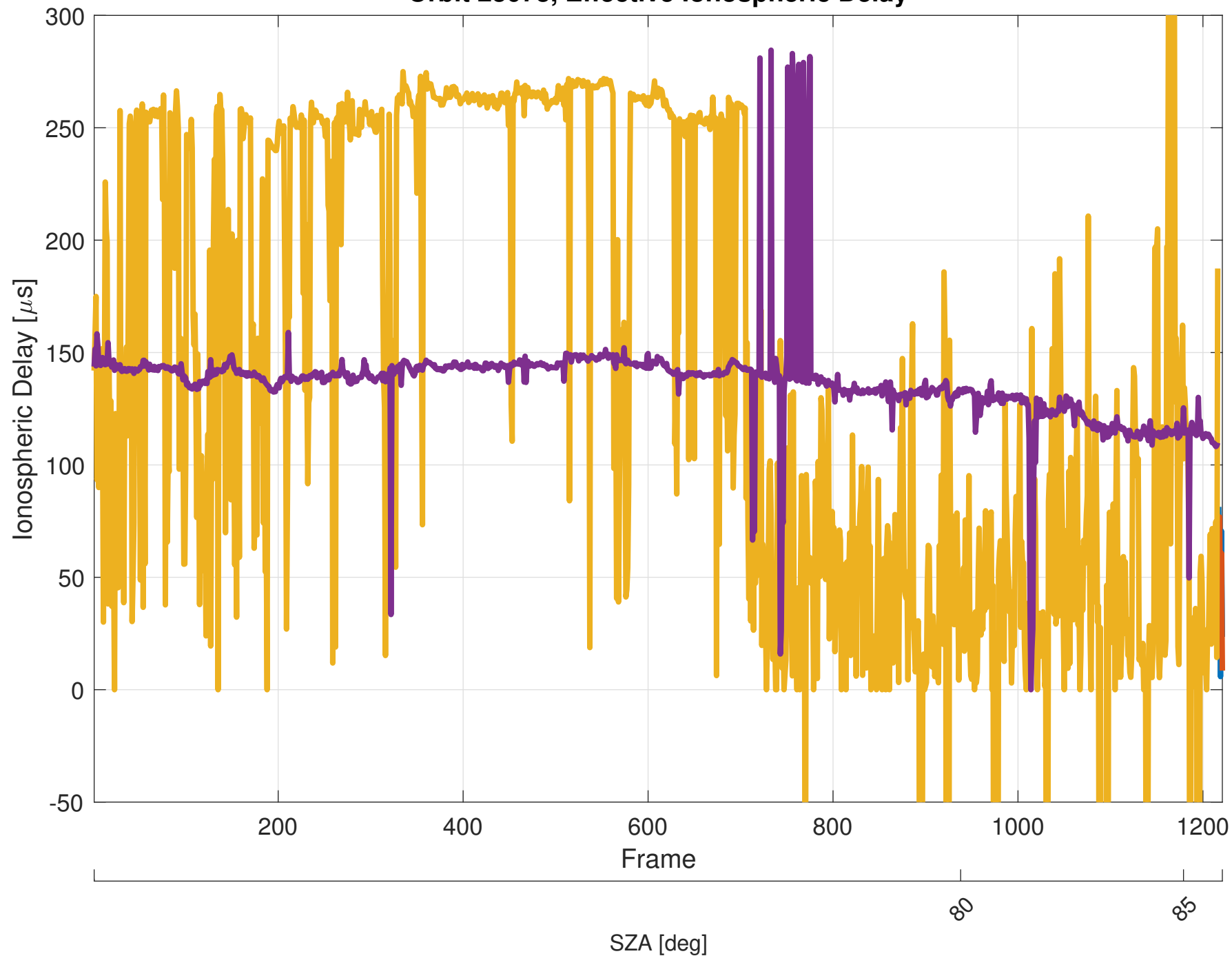
Orbit 23073, Effective Ionospheric Delay
