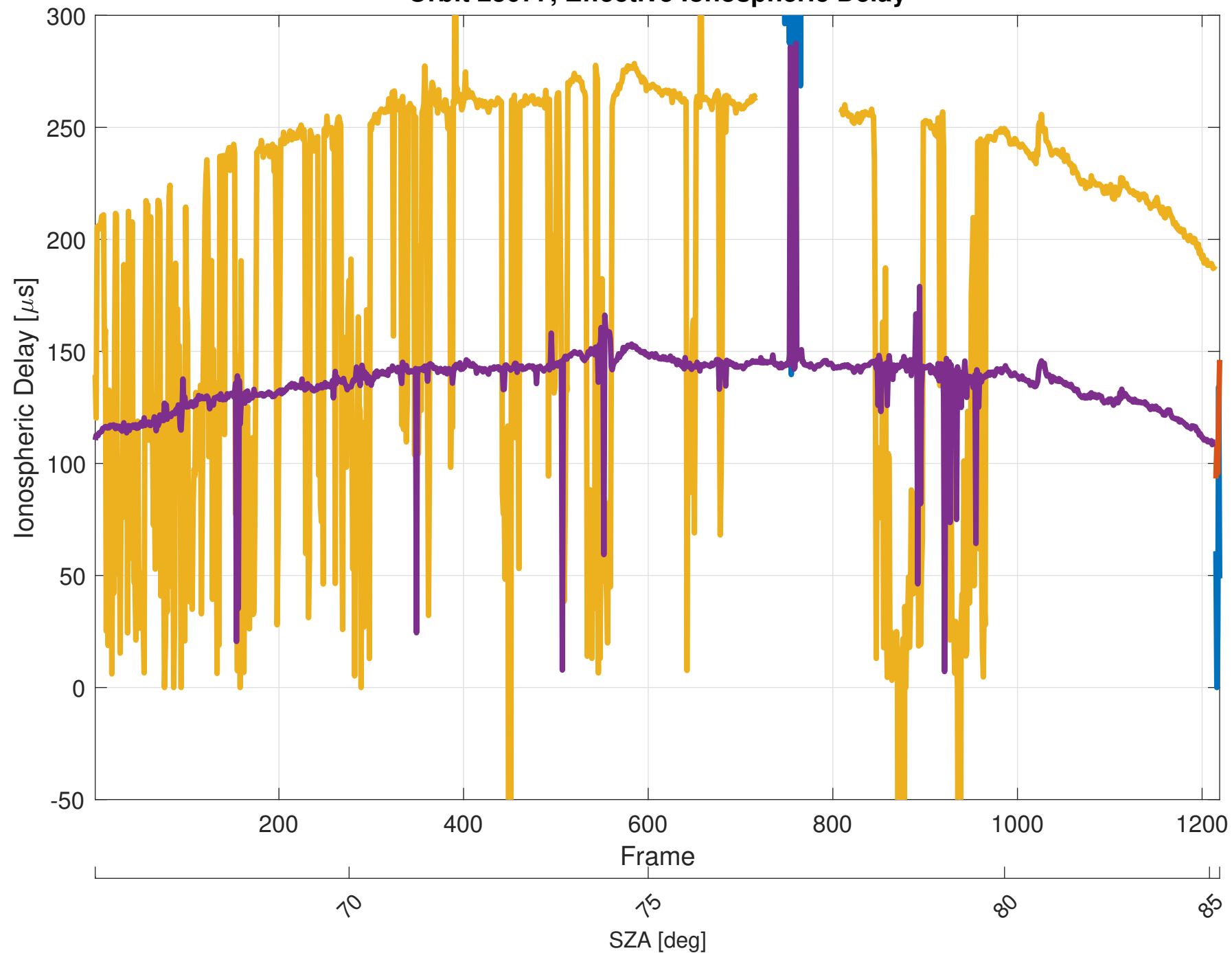
Orbit 23077, Effective Ionospheric Delay
