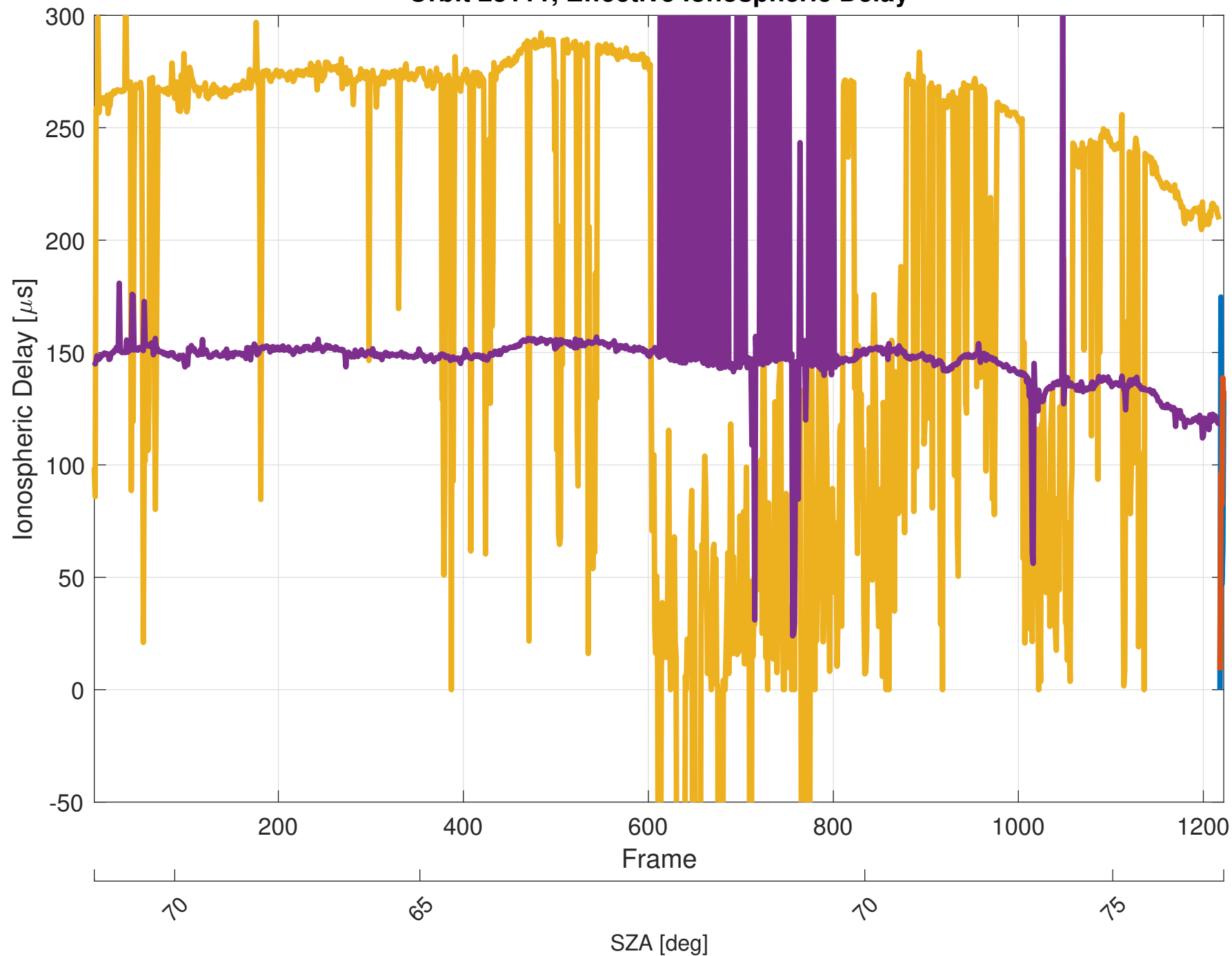
Orbit 23111, Effective Ionospheric Delay
