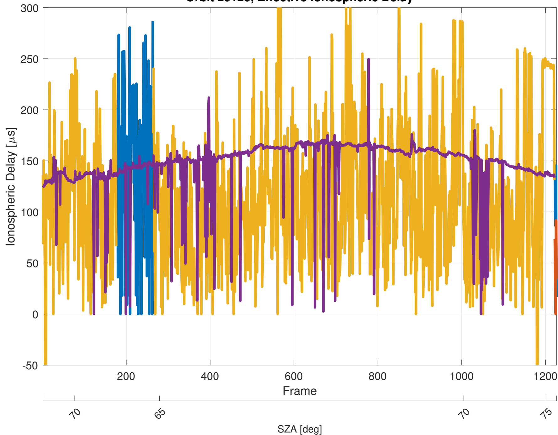
Orbit 23123, Effective Ionospheric Delay
