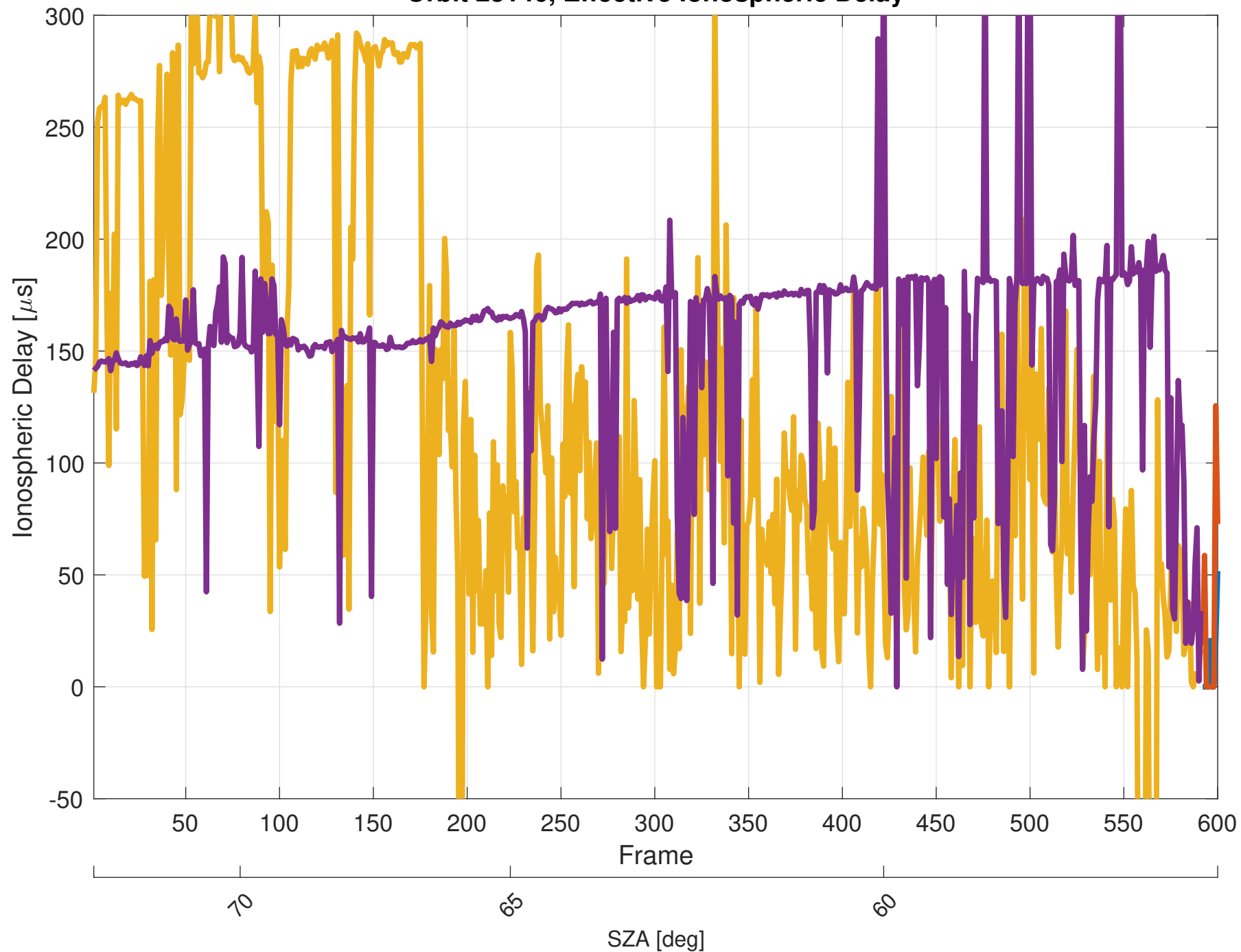
Orbit 23146, Effective Ionospheric Delay
