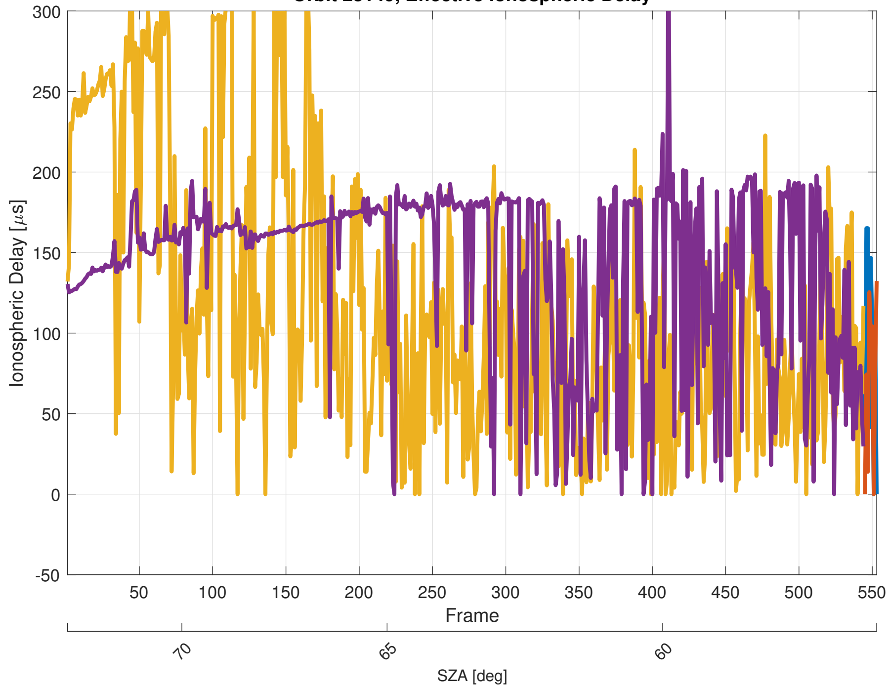
Orbit 23149, Effective Ionospheric Delay
