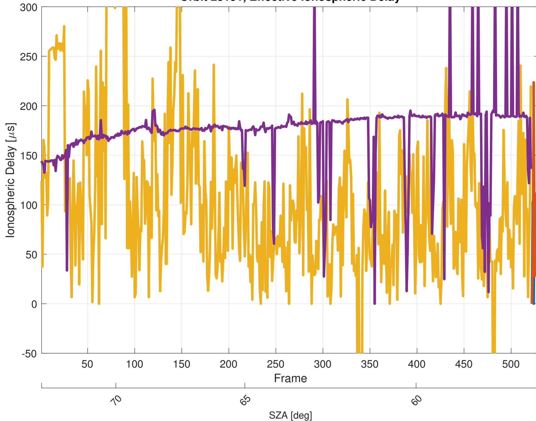
Orbit 23151, Effective Ionospheric Delay
