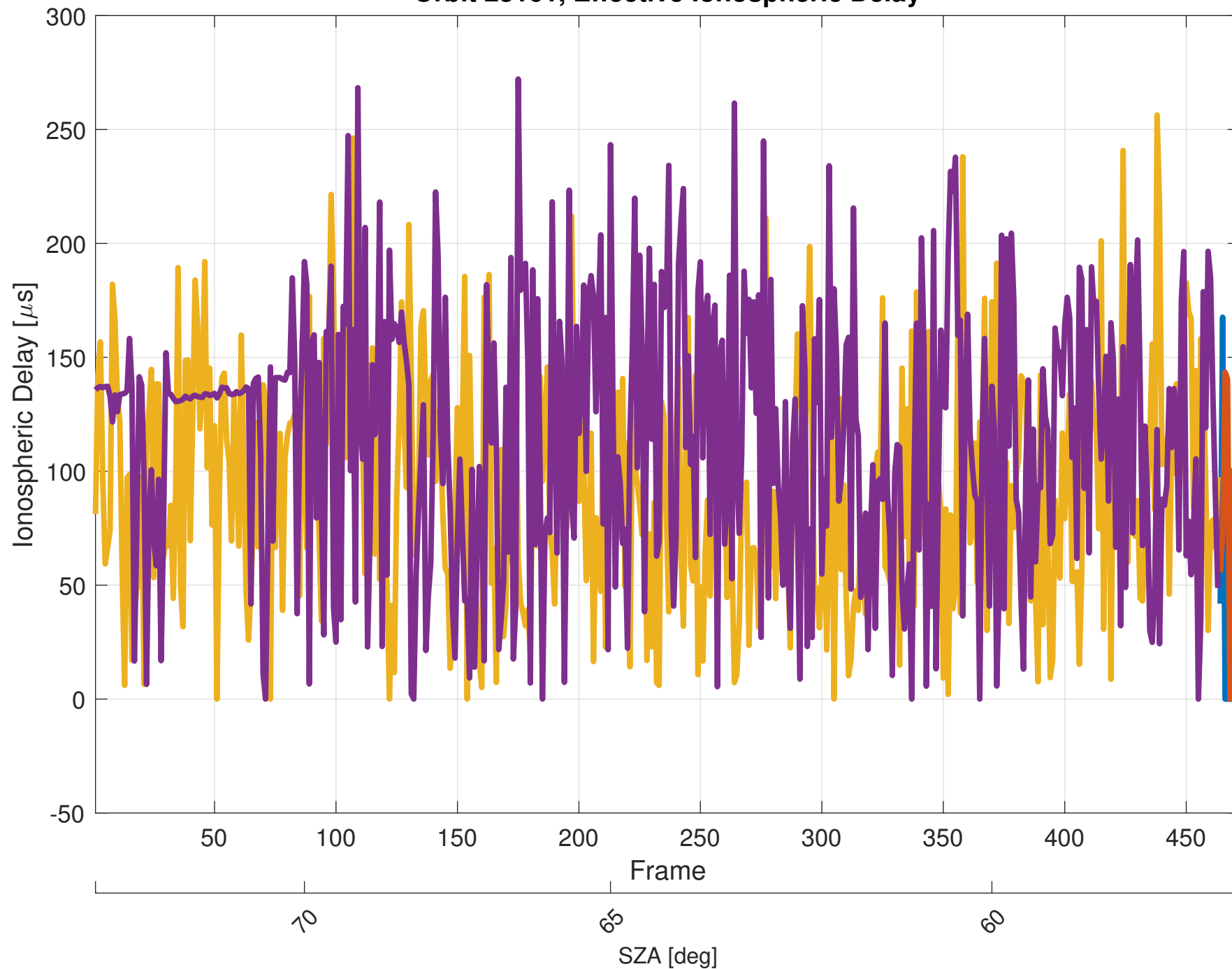
Orbit 23161, Effective Ionospheric Delay
