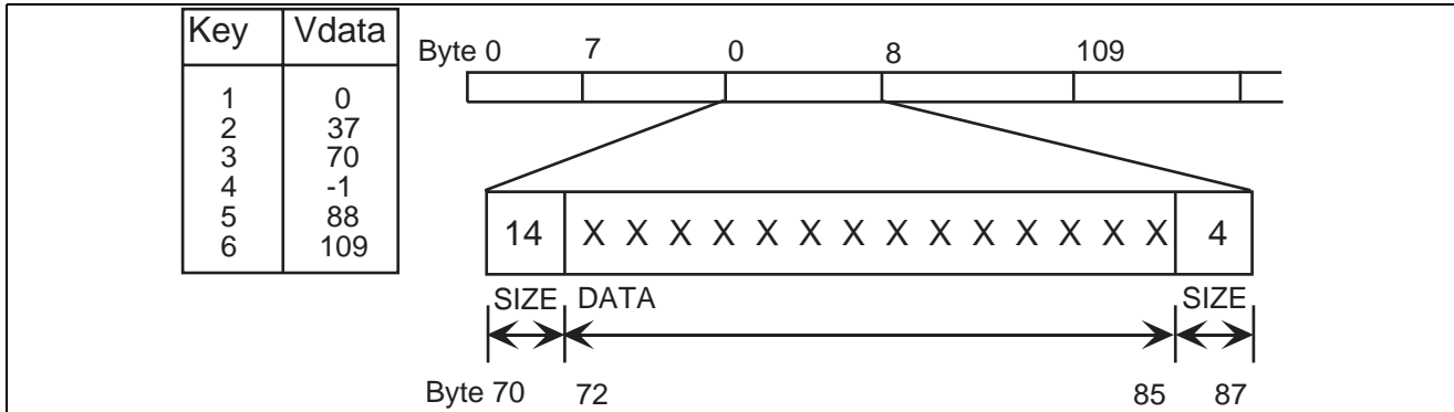
Figure 1. An example of a variable length record.
