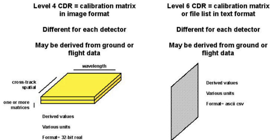
Figure 3-19. Contents of a CRISM Calibration Data Record (CDR). Level 4 is image data; level 6 is text.
