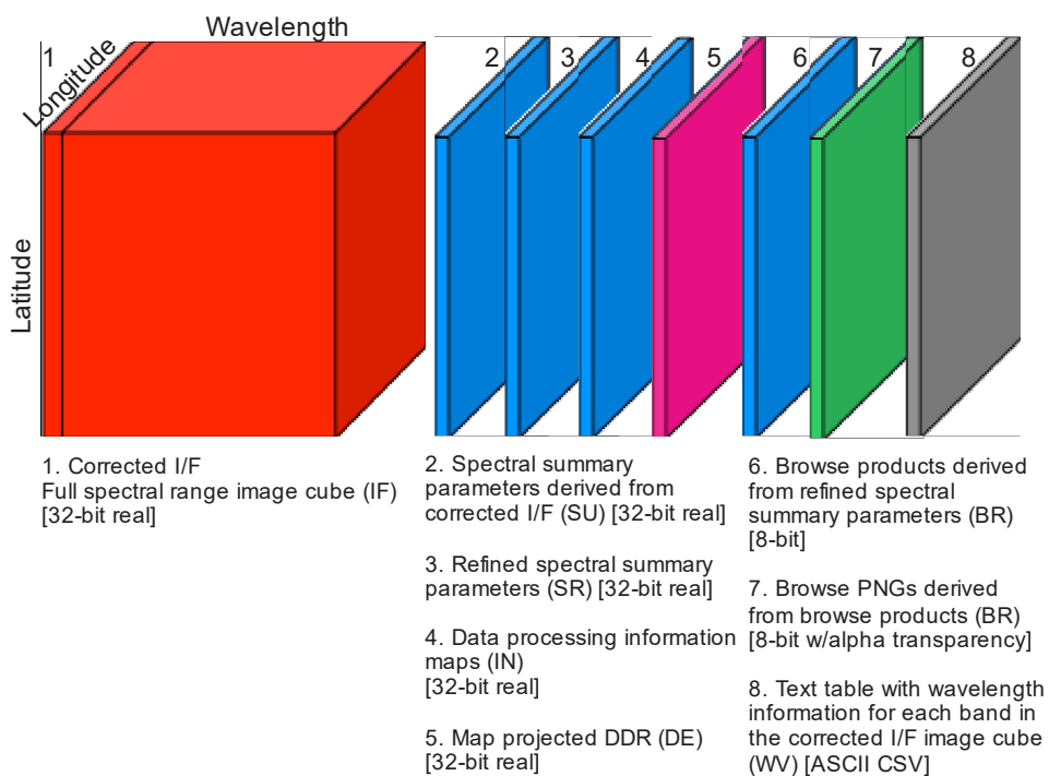
Figure 3-17. Contents of a CRISM Map-projected Targeted Reduced Data Record (MTRDR) Data Product Set
