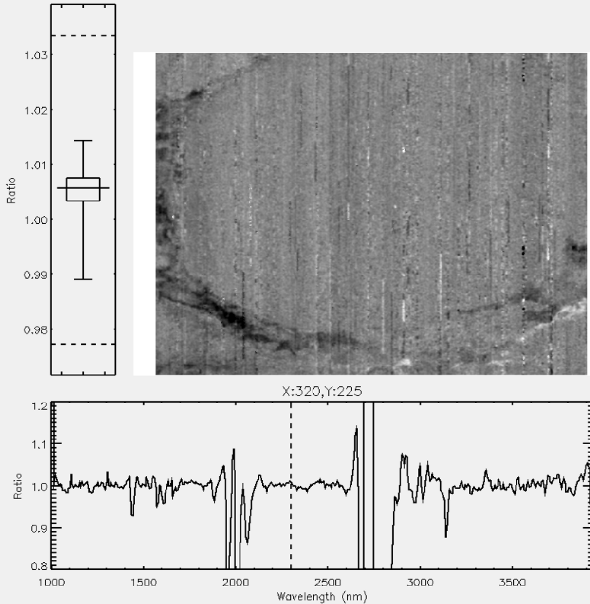
Figure N-6: FRT0000C202 resolve cube. Stochastic noise components have been highly reduced while real high frequency spatial/spectral variability has been retained.
