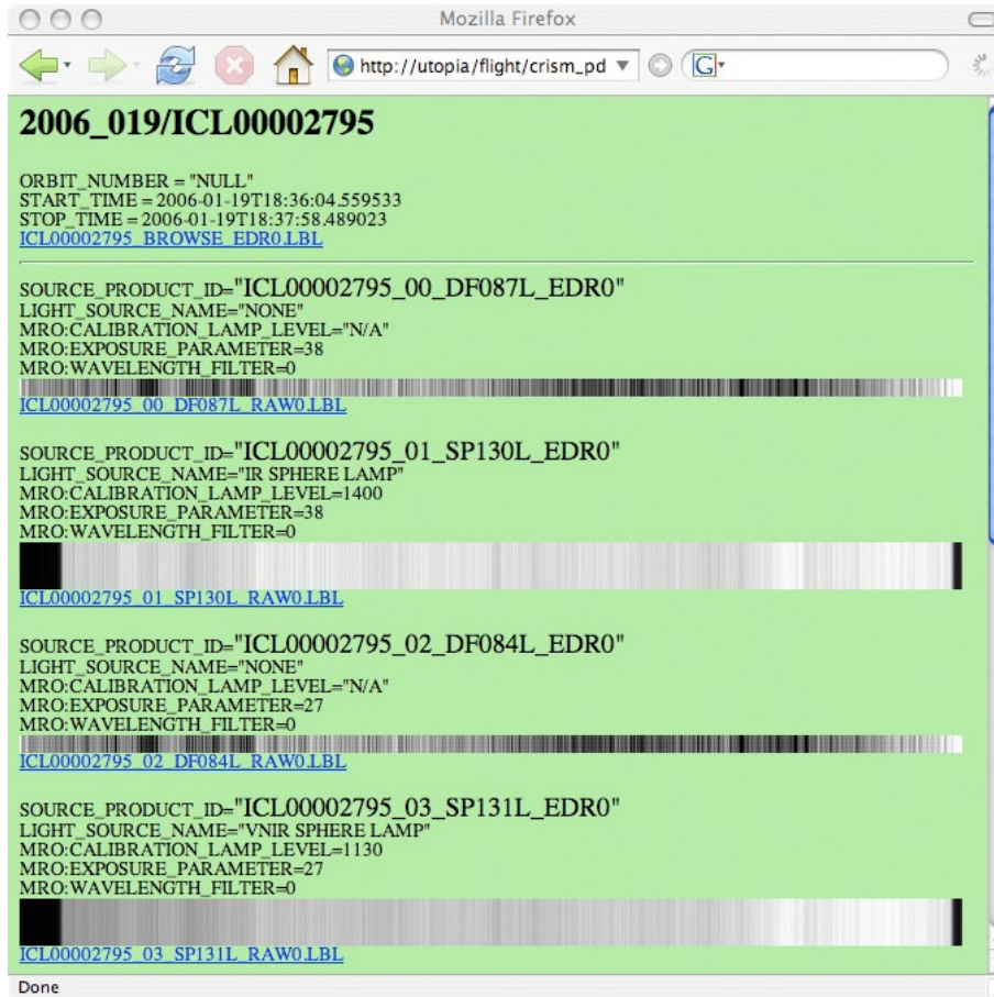
Figure 3-27. Example EDR browse product
