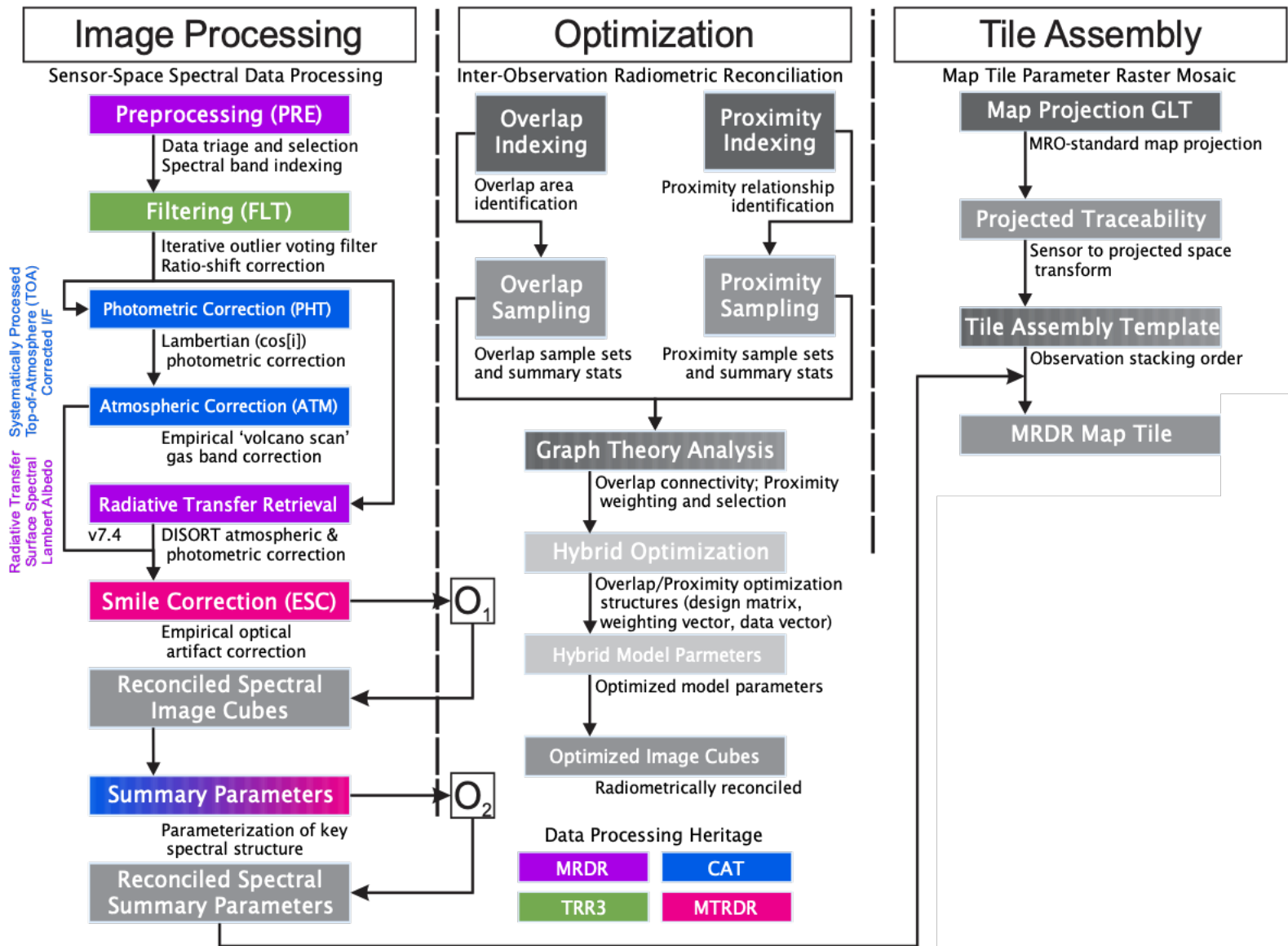
Figure 2-9c Sequential processing of DDRs and TRDRs to create v4 MRDRs.
