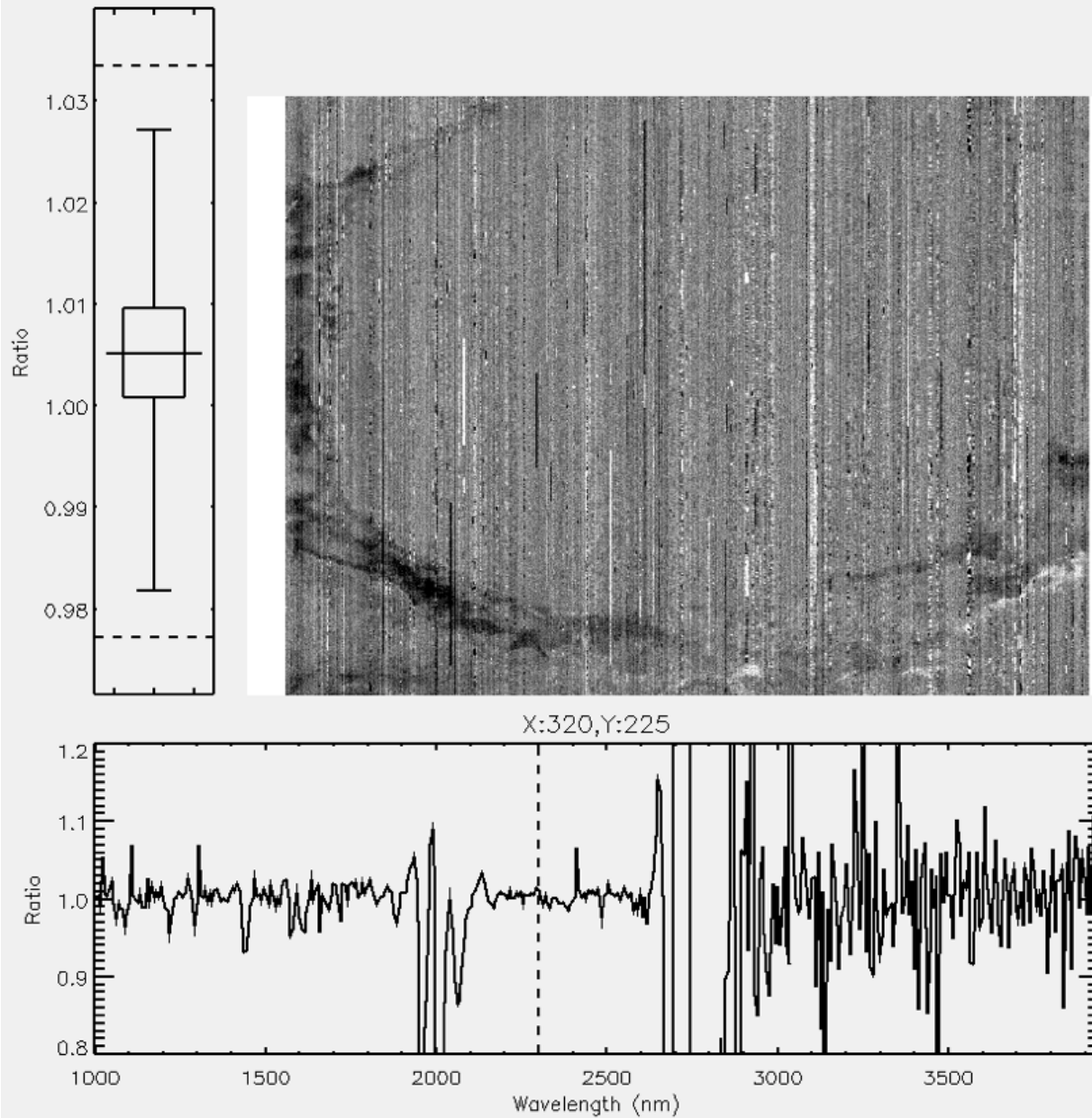
Figure N-4: FRT0000C202 ratio cube. Spatial pixel scale variability due to low-spectral frequency continuum variation is retained by the reference cube (Figure 3) but normalized out of the ratio cube. The ratio cube contains both high frequency noise and high frequency signal components. The spectral plot corresponds to the center pixel in the scene.
