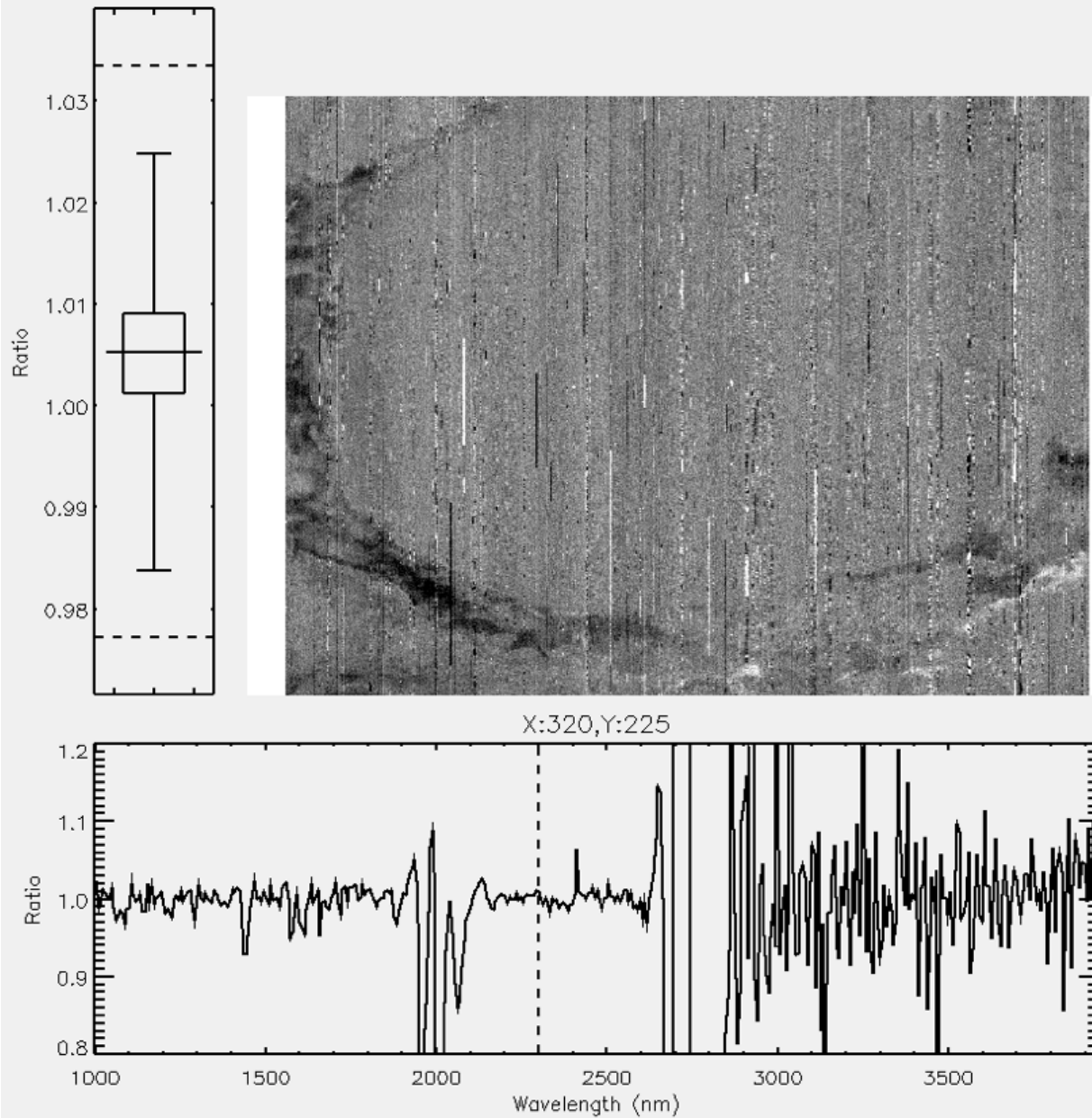
Figure N-5: FRT0000C202 ratio RSC cube. Systematic column-to-column (along track) bias has been mitigated.
