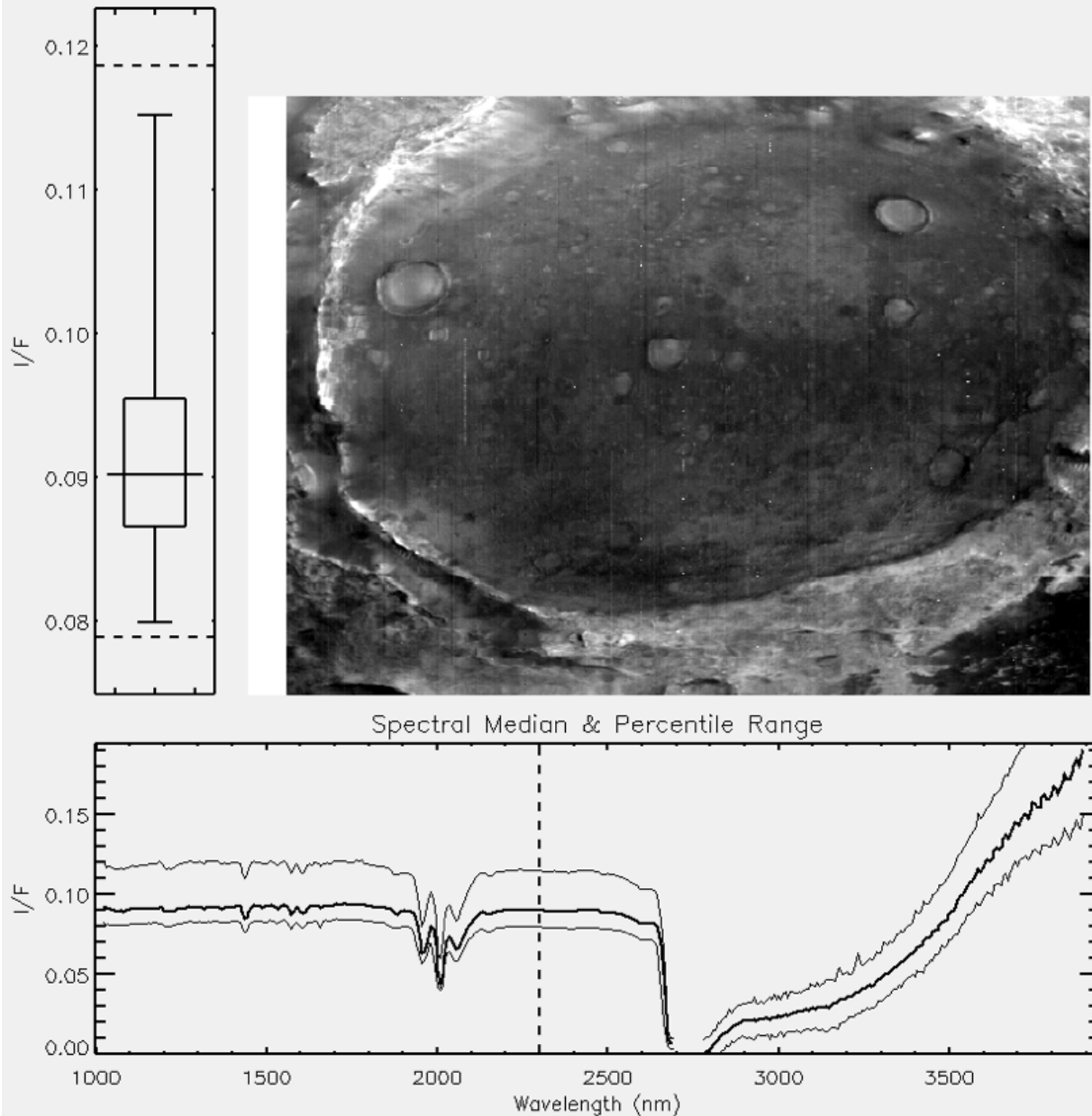
Figure N-2: Three panel composite view of FRT0000C202 segment 0x07 (central scan) input I/F IR image cube. The corresponding radiance image has been delivered to the PDS as FRT0000C202_07_RA165L_TRR3.IMG Observation FRT0000C202 was acquired with an IR detector temperature of \sim 120.8 K. The systematic and stochastic noise components to be addressed by the filtering procedure are evident as bright pixels and vertical lines. The composite plot consists of: 1) Band 240 ( \sim 2300 nm) ground plane (x,t) image with a 1% linear stretch; 2) Boxplot showing the data distribution and stretch limits for the displayed band; 3) Median spectrum and [1,99]% envelope for the input image cube.
