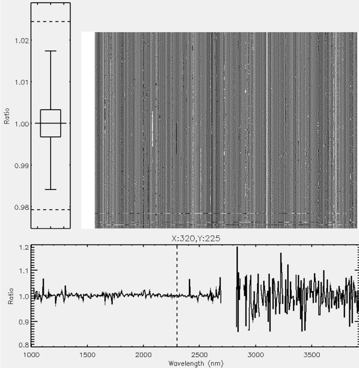
Figure N-9: FRT0000C202 input / output ratio cube showing the effect of the data filtering procedure. Note that the single pixel input/output ratio spectrum and band 240 ratio data are centered on unity.
