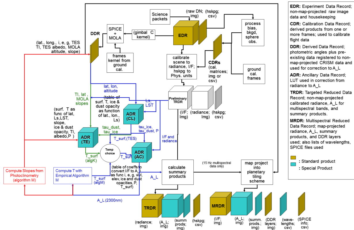
Figure 2-9a. Sequential processing of EDRs to yield RDRs of Mars data, showing the roles of CDRs and ADRs.
