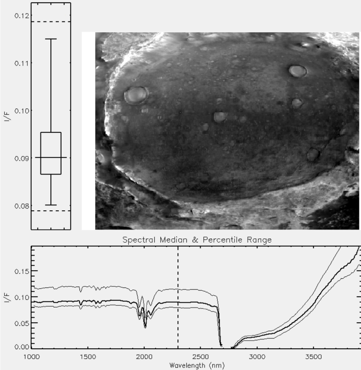
Figure N-8: FRT0000C202 restore cube – delivered to the PDS as FRT0000C202_07_IF165L_TRR3.IMG. Compare the ground plane image, median spectrum and spectral percentile envelope, and data distribution boxplot to Figure 2.
