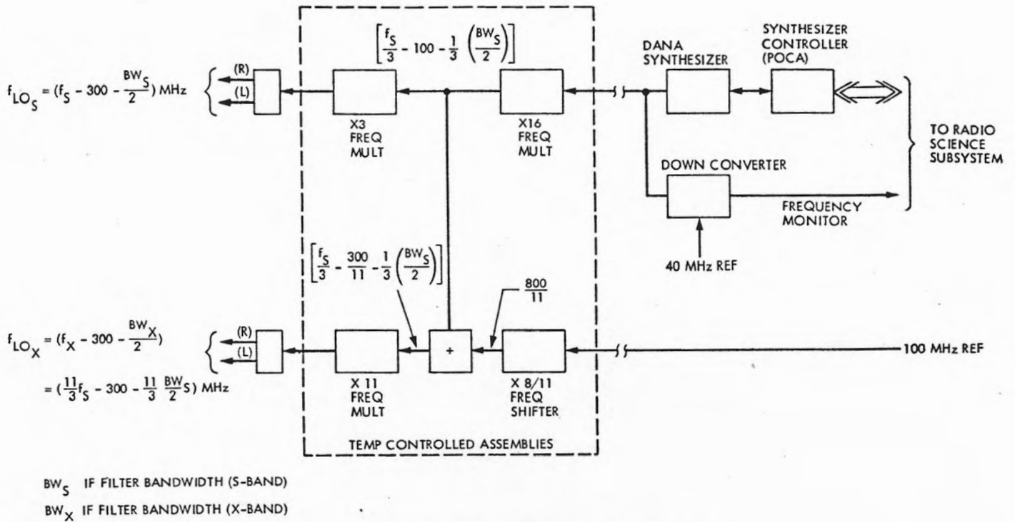
Fig. 5. Occultation channels – first local oscillator
