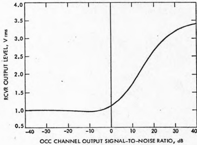
Fig. 6. OCC channel operating level
