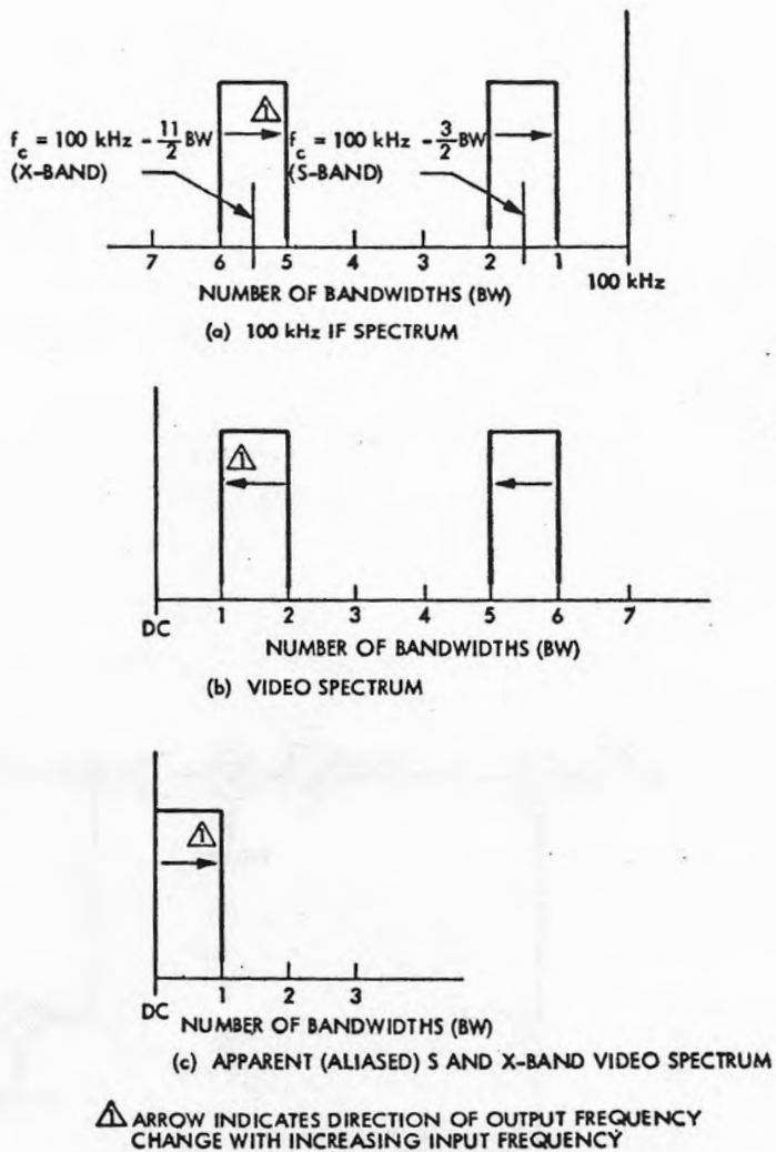
Fig. 4. Very narrow band filter channel spectrum: (a) 100-kHz IF spectrum, (b) video spectrum, (c) apparent (aliased) S- and X-band video spectrums
