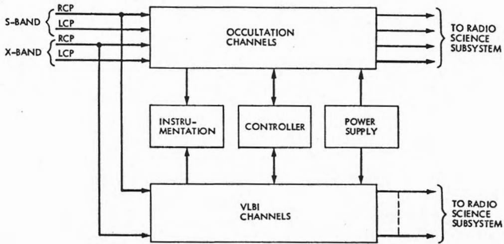
Fig. 1. Multi-Mission Receiver
