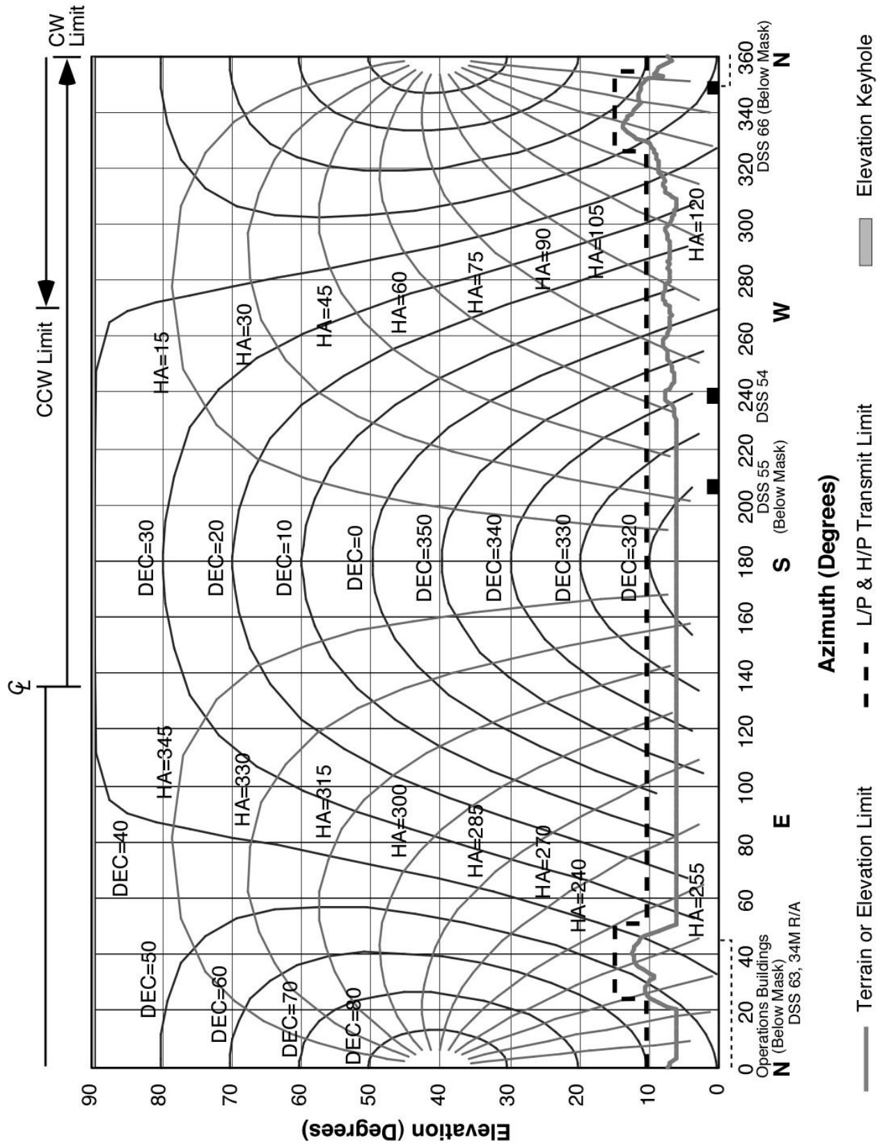
Figure 23. DSS 65 Hour-Angle and Declination Profiles and Horizon Mask
