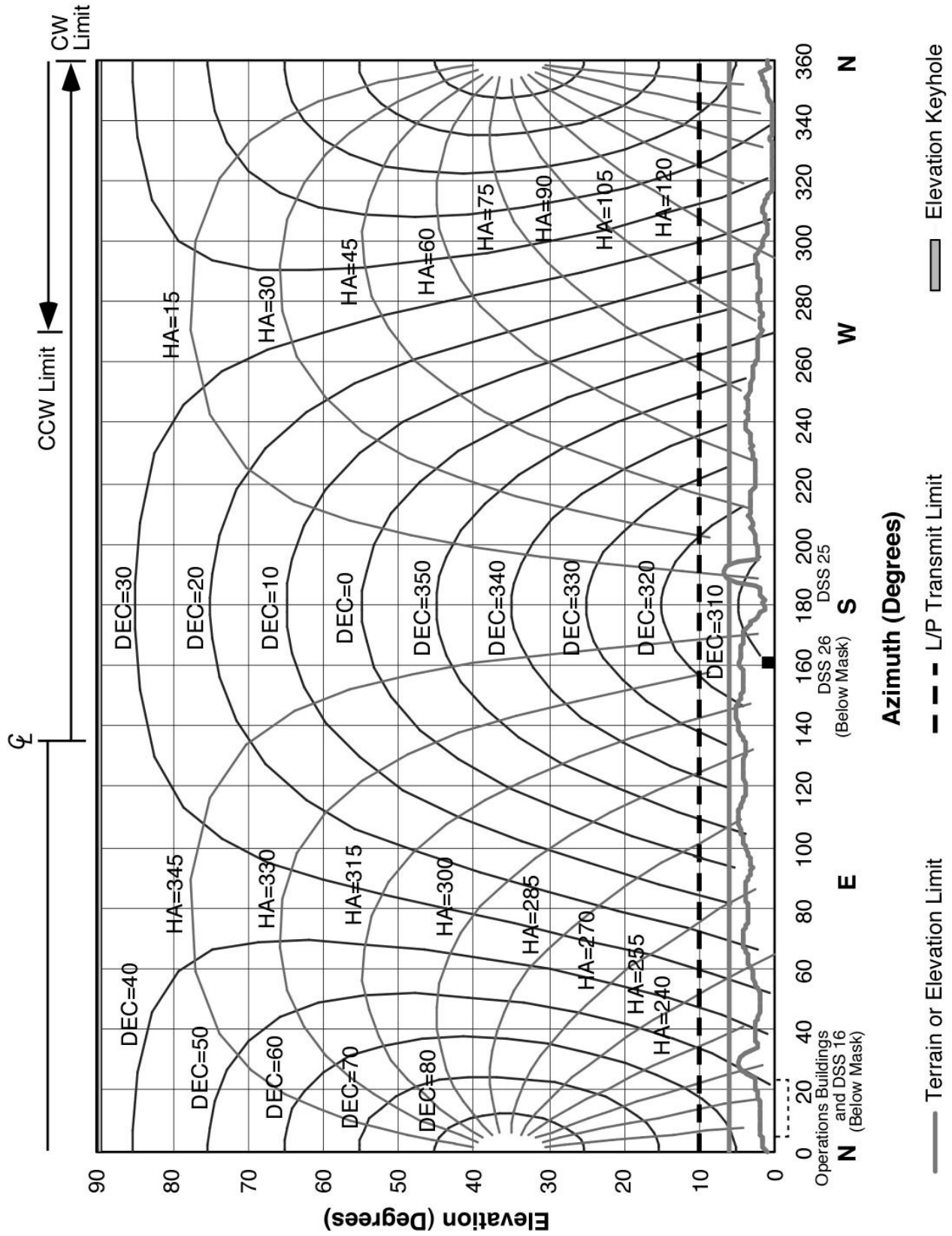
Figure 13. DSS 24 Hour-Angle and Declination Profiles and Horizon Mask
