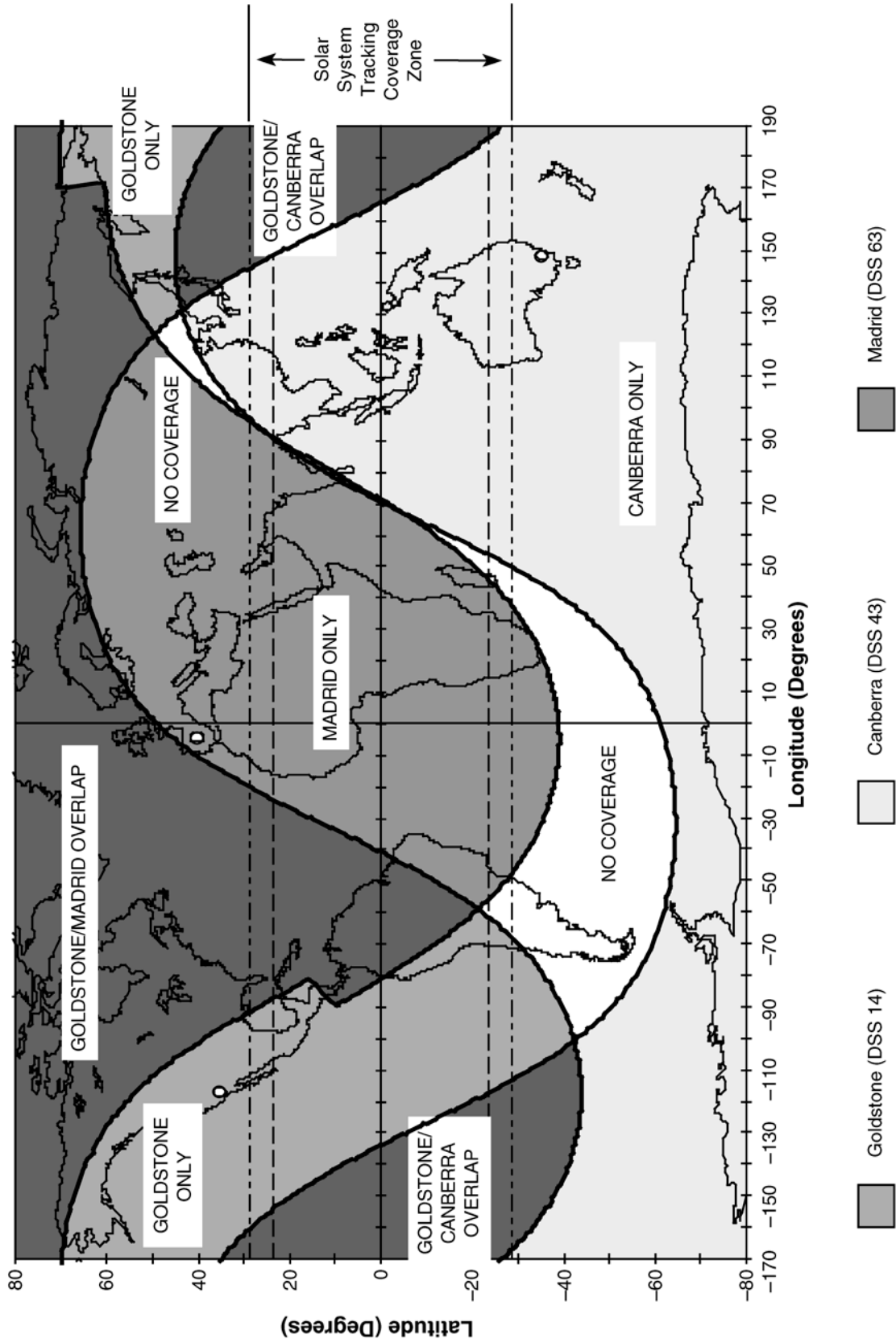
Figure 3. DSN 70-m Subnet Transmit Coverage, Planetary Spacecraft.
