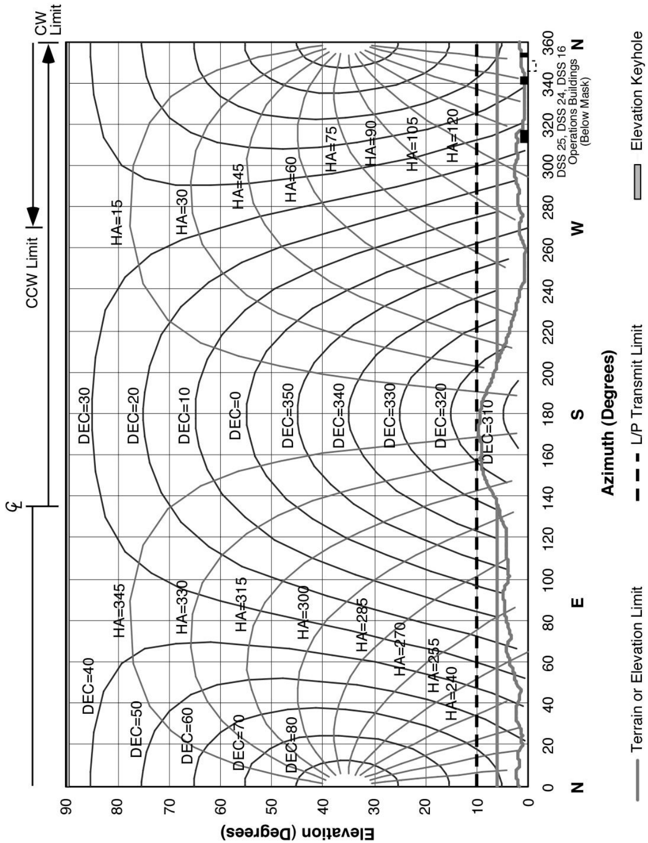
Figure 15. DSS 26 Hour-Angle and Declination Profiles and Horizon Mask
