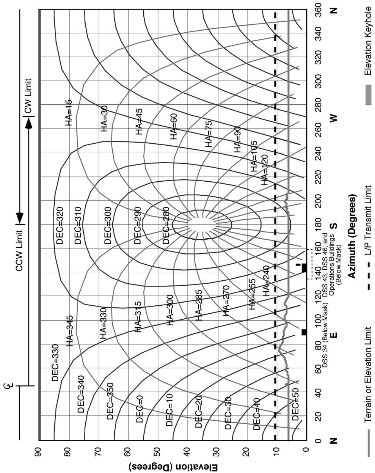
Figure 19. DSS 45 Hour-Angle and Declination Profiles and Horizon Mask
