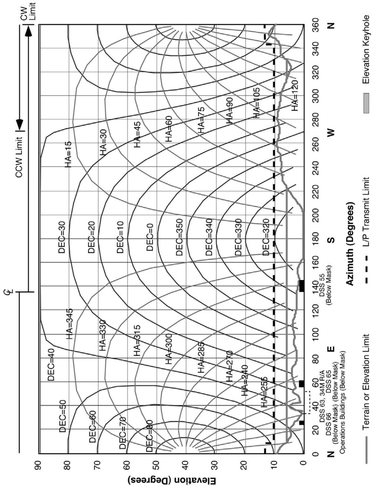
Figure 20. DSS 54 Hour-Angle and Declination Profiles and Horizon Mask
